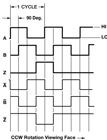
Figure 1 Output Waveform
